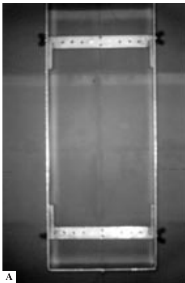
Figure 3 (A and B) Bottomless, lidless metal box (A) used to position rats to be radiographed. The box has two runners and two metal rods parallel to each other on the horizontal and sagittal planes (B).
